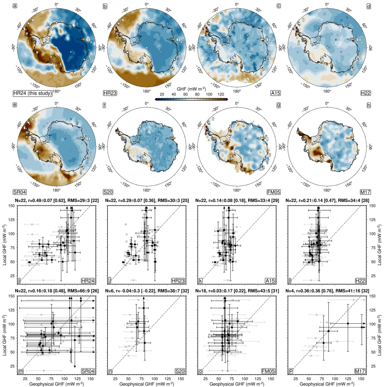
Figure 4. GHF Model Comparison. (a–h) Geophysical GHF inferences: HR24— inferred directly from V_S and V_P (this study); HR23— inferred directly from V_S (Hazzard et al., 2023); A15— inferred directly from V_S (An et al., 2015); H22— inferred via joint seismic and gravity inversion (Haeger et al., 2022); SR04— inferred empirically via V_S (Shapiro & Ritzwoller, 2004); S20— inferred empirically via V_S (Shen et al., 2020); FM05— inferred from magnetic anomaly data (Maule et al., 2005); M17— inferred from magnetic anomaly data (Martos et al., 2017). GHF inferences derived from gravity-driven probes and boreholes overlay as colored capsules/circles . Capsules used where 2+ local data points available (colored by lowest-average-highest local estimate from bottom-middle-top). Circles used where 1 local data point available. Note that HR24 has been extended into the oceanic domain to allow more complete comparison with local data. In the oceanic domain we assume k_0 = 2.6 \text{ W m}^{-1} \text{ K}^{-1} and h_{cu}^* = 0.0 \text{ } \mu\text{W m}^{-3} , in keeping with oceanic crustal composition (Grose & Afonso, 2013; Richards et al., 2018). (i–p) Relationship between geophysically and locally inferred GHF (Section 3.3), same studies as (a–h). Data points and associated error bars show the mean and range of local/geophysical GHF values at each location, respectively. Statistics summarizing local-geophysical agreement are: r = Pearson's r -value correlation coefficient; RMS = root-mean-square deviation (values reported in the form a \pm b [c] , where a = median, b = median absolute deviation, c = value calculated ignoring data uncertainty, see Text S5 in Supporting Information S1 for details of analysis). Gray data points correspond to locations where only one local GHF inference is available (i.e., circles in panels (a–h)) and are not included in model statistics.
