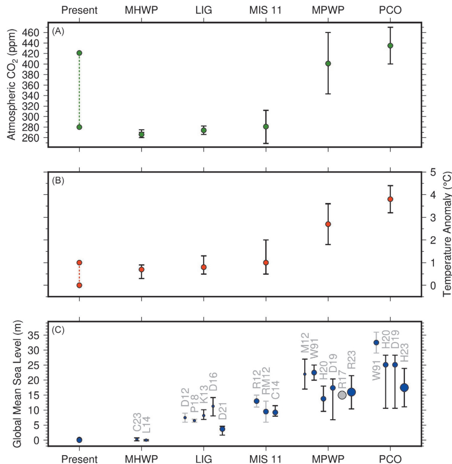
Fig. 5 Summary of climatic variables during key warm periods. (A) Atmospheric CO 2 (Brovkin et al., 2016; Rae et al., 2021). Dotted lines connect between preindustrial and present-day conditions. (B) mean global surface temperature (Burke et al., 2018; Rachmayani et al., 2017; Tzedakis et al., 2022; Brierley and Fedorov, 2010). (C) GMSL. Gray symbol/blue with gray error bar/blue with black error bar = no/limited/comprehensive uncertainty quantification; small/medium/large symbol = uncorrected/indirectly corrected/directly corrected for dynamic topography-induced RSL changes. C23 = (Creel et al., 2022); L14 = (Lambeck et al., 2014); D12 = (Dutton and Lambeck, 2012); P18 = (Polyak et al., 2018); K13 = (Kopp et al., 2013); D16 = (Düsterhus et al., 2016); D21 = (Dyer et al., 2021); R12 = (Roberts et al., 2012); RM12 = (Raymo and Mitrovica, 2012); C14 = (Chen et al., 2014); M12 = (Miller and Becker, 2012); W91 = (Wardlaw and Quinn, 1991); H20 = (Hearty et al., 2020); D19 = (Dumitru et al., 2019); R17 = (Moucha and Ruetenik, 2017); R23 = (Richards et al., 2022); H23 = (Hollyday et al., 2023).
